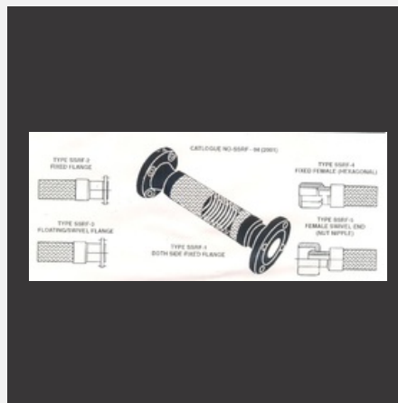
Corrugated Metallic Flexible Hose
